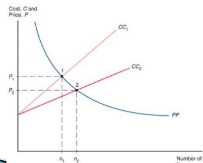
Fig. 8-4: Effects of a Larger Market
