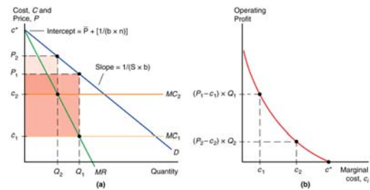
Fig. 8-6: Performance Differences Across Firms
