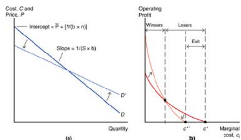
Fig. 8-7: Winners and Losers from Economic Integration
